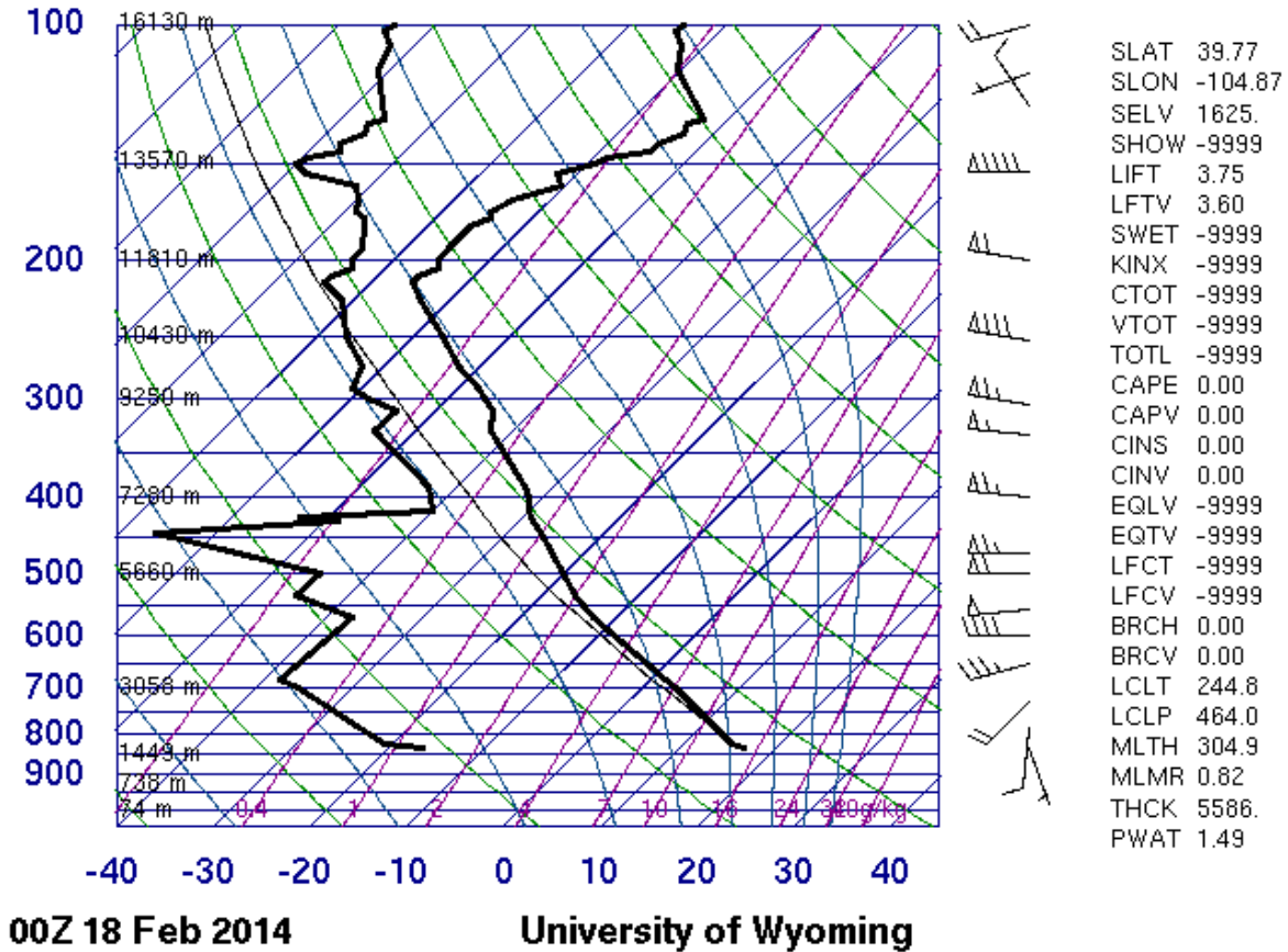
Figure 3 Skew-T plot for February 18, 2014
