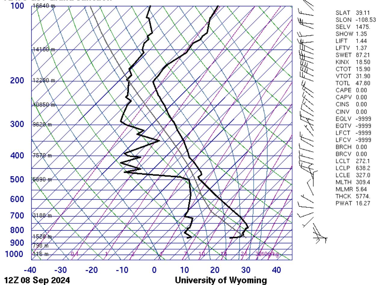
Figure 3.0.1: Grand Junction, CO Skew-T diagram for September 8th, 2024
