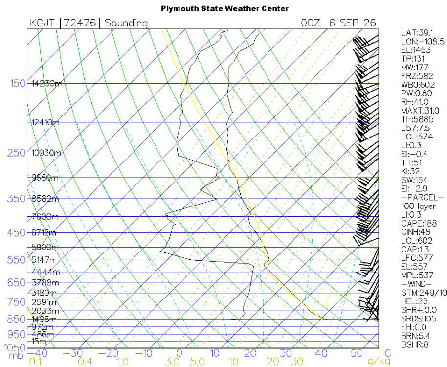
Figure 1: Sounding data from GJT on September 6 at 00Z.
